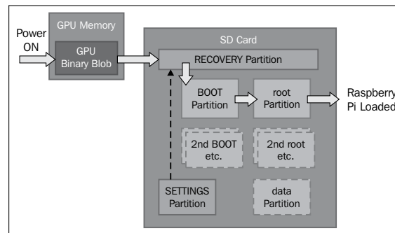
NOOBS creates several partitions on the SD card to allow installation of multiple operating systems and to provide recovery
